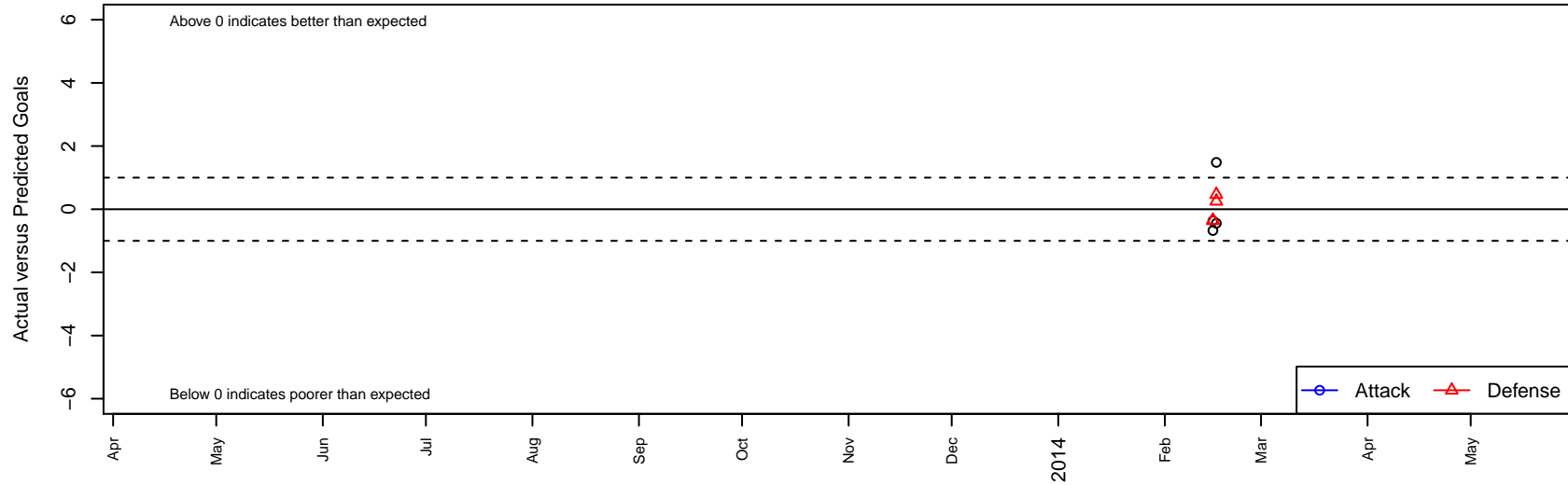
FC Blazers B00 Dots are actual minus expected GF (blue circles) and GA (red triangles). Blue line is smoothed change in attack strength. Red is smoothed change in defense strength.
